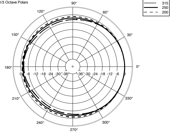
Vertical 1/3 Octave Polars
