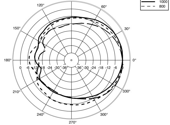
Vertical 1/3 Octave Polars
